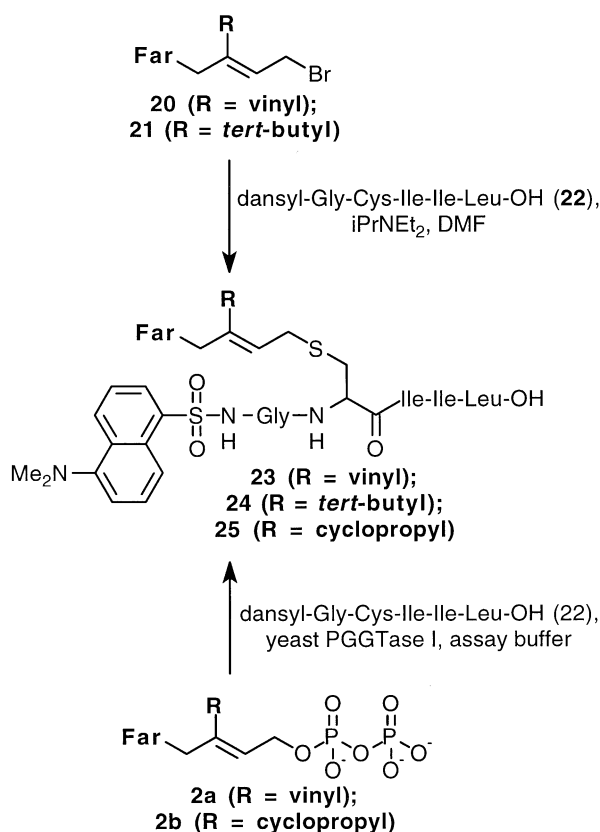
Scheme 5.
